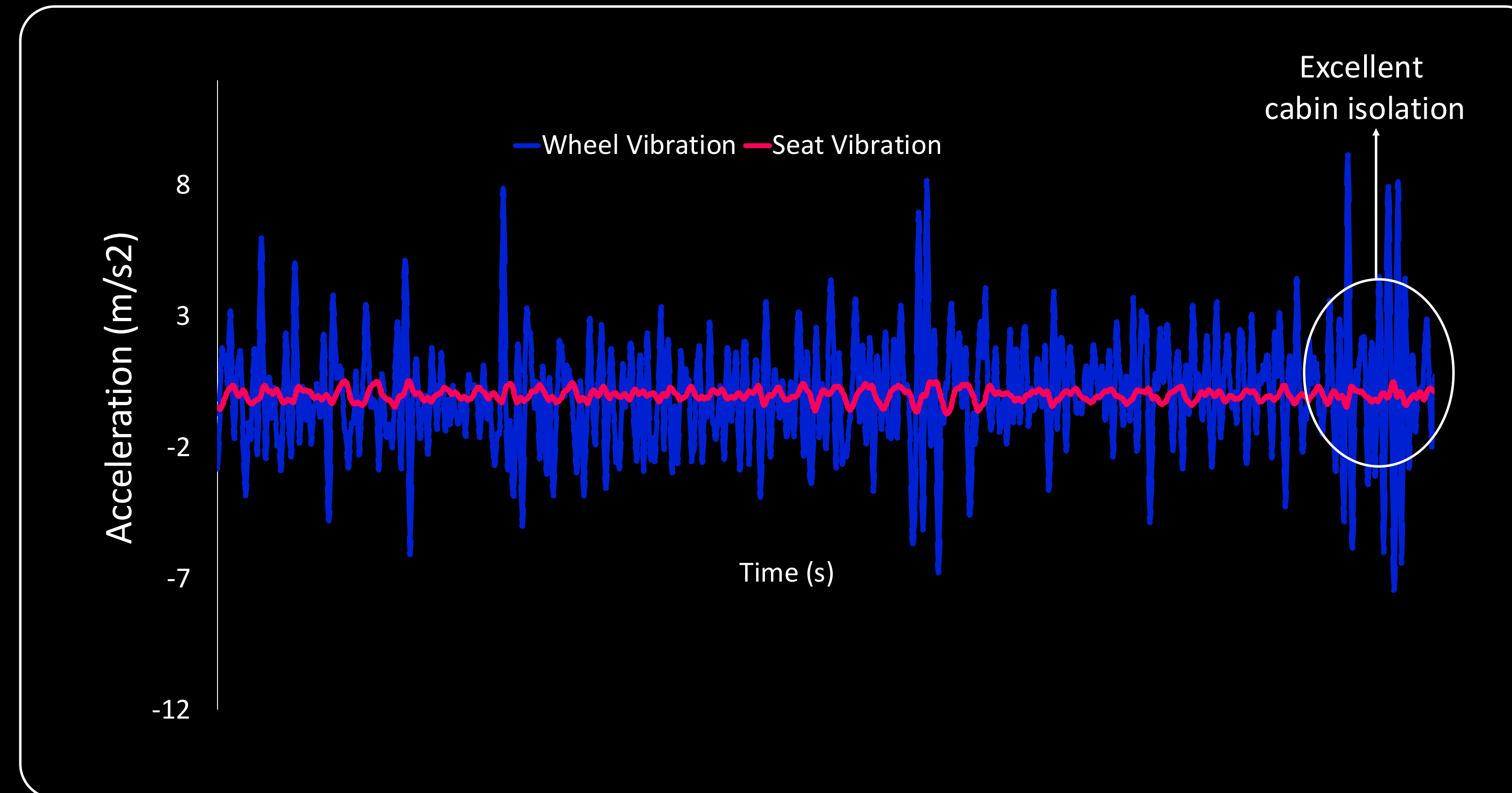
Ride comfort – Road inputs isolation
