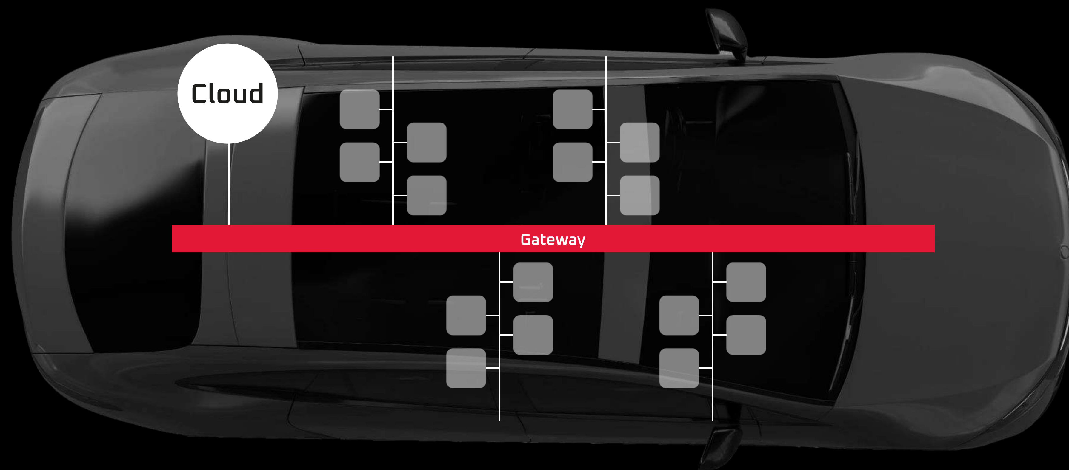
Typical Distributed Architecture
