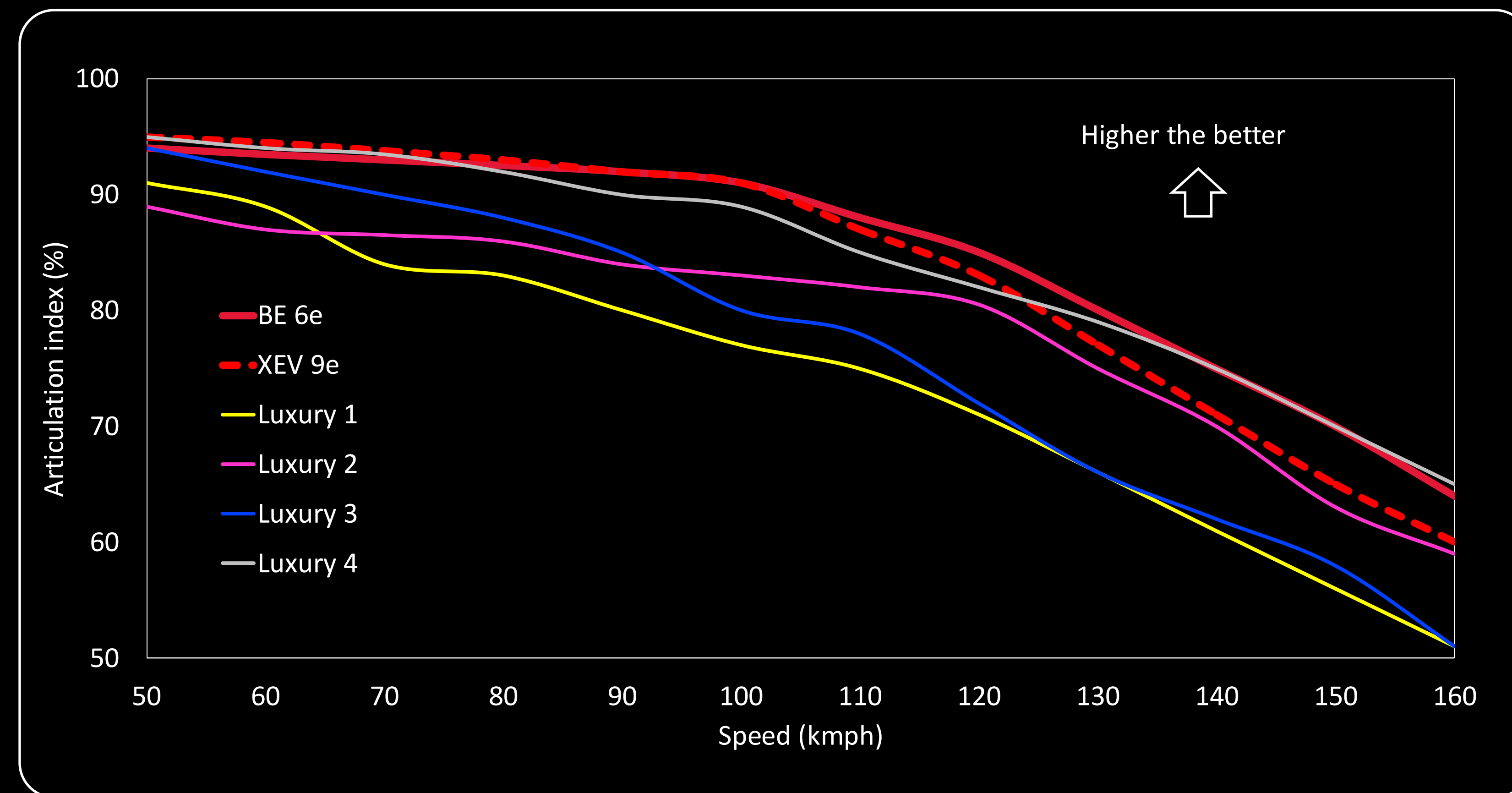
Articulation Index (Sound Quality) Driver-ear noise
