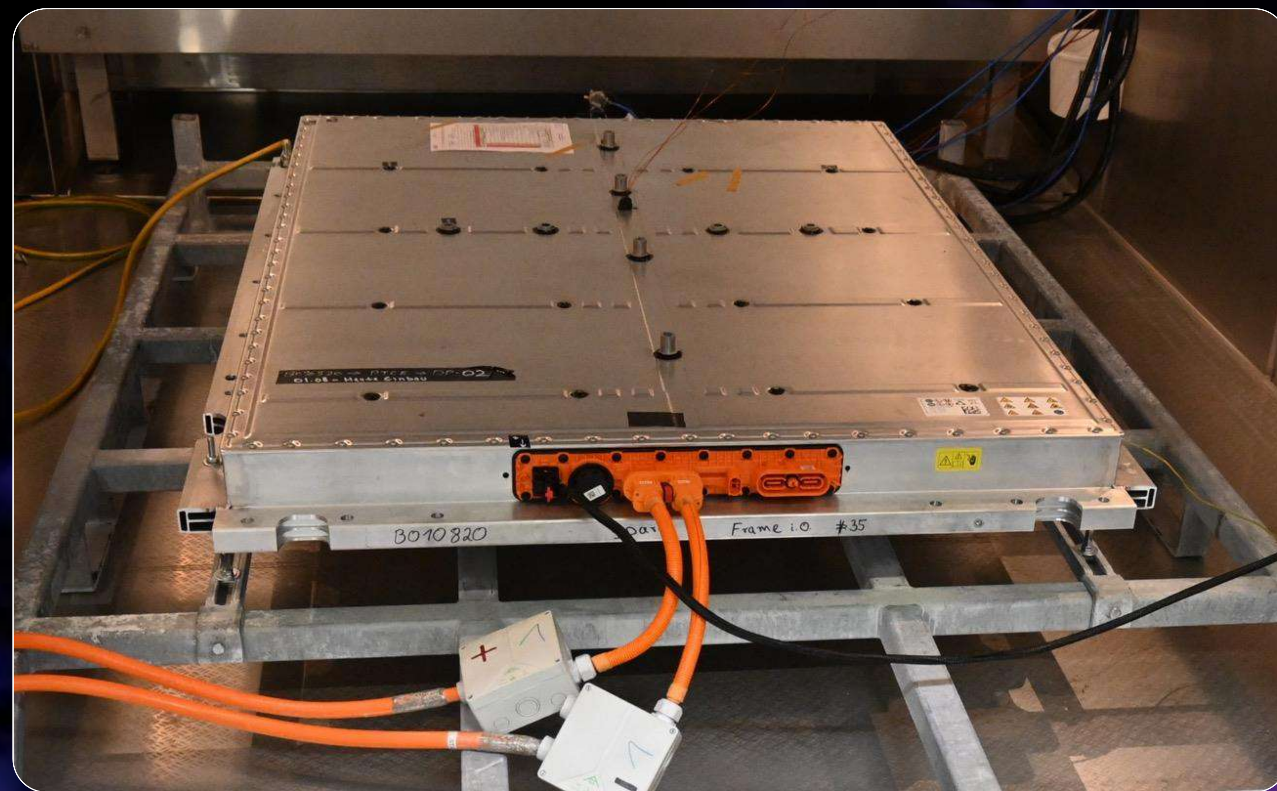
HV safety
